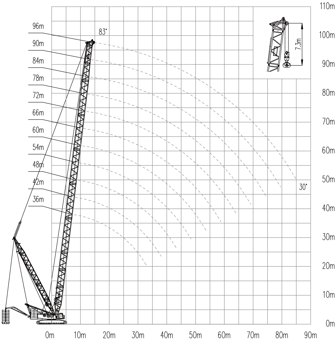
7. Superlift heavy boom working condition (SHB)
